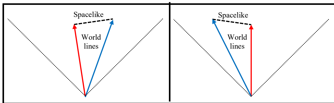
Figure 2 – Poincaré Rotations : Left panel, observer moving to the left; right panel, observer moving to the right. While the light cones don't change, the timelike and spacelike intervals do. Neither observer sees detections of these two objects as simultaneous. However, the 'length' of the spacelike interval (measured in Minkowski space, where the time dimension is imaginary) is an invariant. The object world lines have been color coded in accordance with their Doppler shifts (red or blue shifted).
