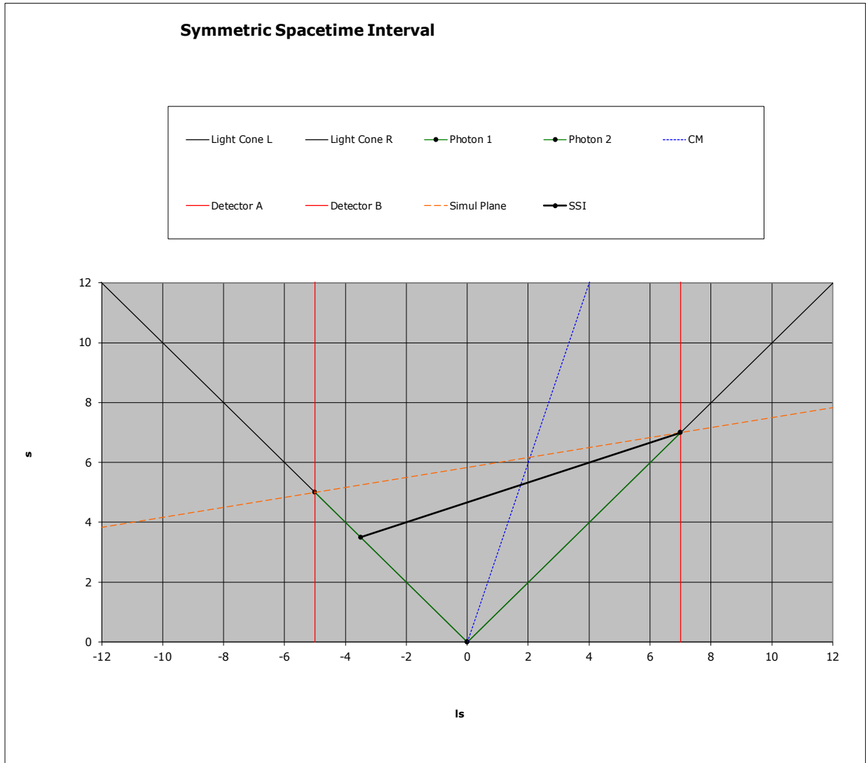
Figure 2 – Symmetric Spacetime Interval for EPR Photons: Vertical lines are the detectors, timelike dashed line the center of mass of the entangled photons, spacelike dashed line the plane of simultaneity for their simultaneous detection, and the spacelike solid line is their symmetric interval. There are four events of interest, indicated by dots; creation - the emission of the entangled photons at (0, 0), encounter - the detection of the first one (on the right) as the symmetric interval encounters the right detector first at (7, 7), responder - the collapse of the second photon (on the left) at the opposite end of the symmetric interval at (-3.5, 3.5) because the other photon was measured, and the validation - the detection of the second photon (on the left) at (-5, 5).
